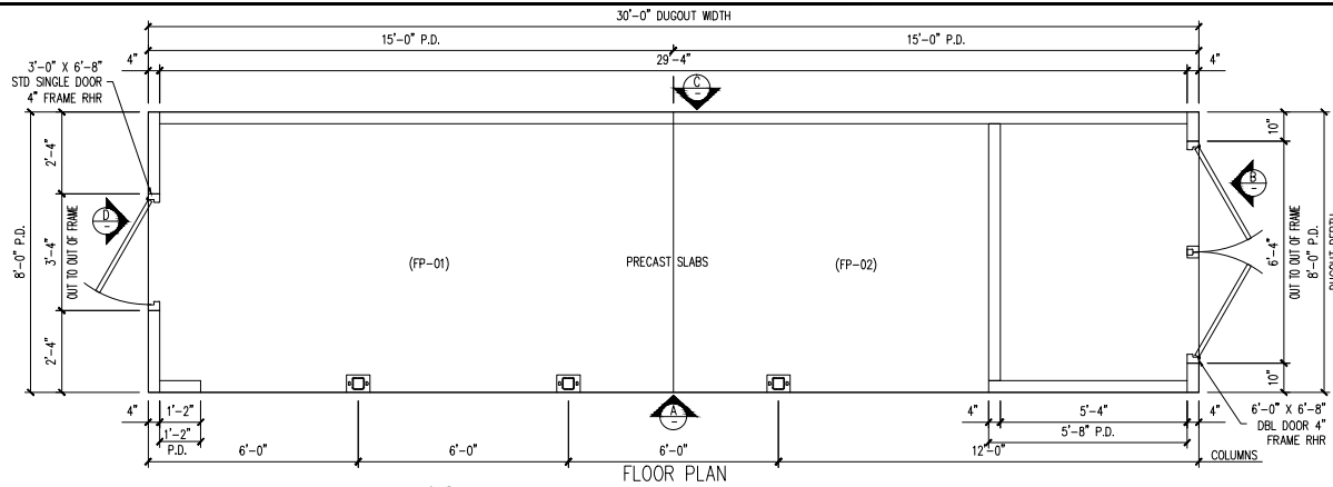
FLOOR PLAN
