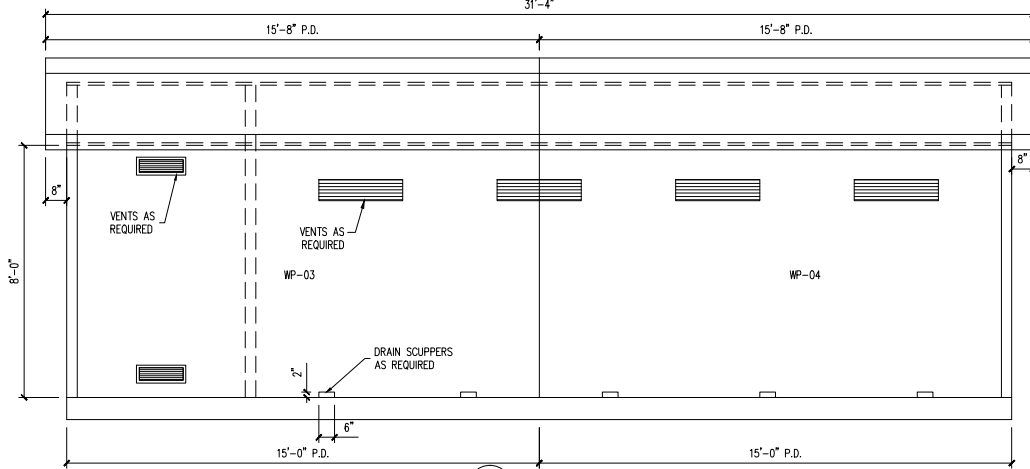
(C) REAR ELEVATION
