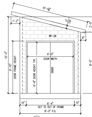
(B) RIGHT ELEVATION
